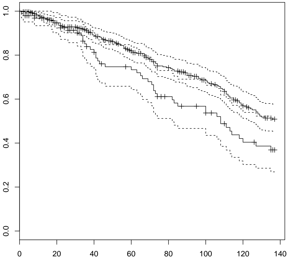
male and female survival curves--Channing data
